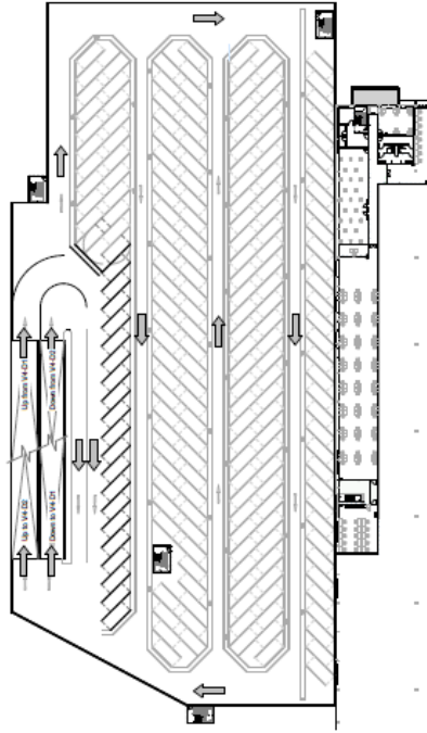
Proposed V4-01 Level 1:100
