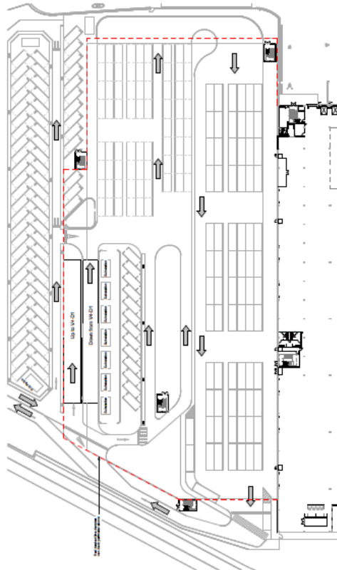
Proposed Ground floor Van Deck Plan 1:100
